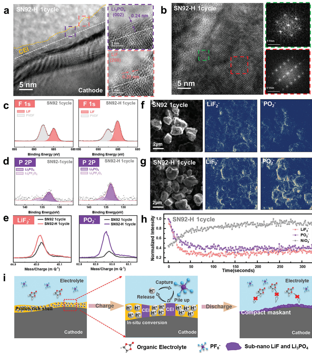
Figure 3. Morphology and composition characterization of the maskant. a) The cryo-TEM images of SN92-H. b) The high-resolution TEM images of the SN92-H and the corresponding FFT among different areas. c, d) The XPS spectra with the same intensity scale of F 1s (c) and P 2p (d) for SN92 and SN92-H. e) TOF-SIMS spectra of LiF 2 - (left) and PO 2 - (right) on SN92 and SN92-H. f, g) Chemical mapping of LiF 2 - and PO 2 - for the electrode of SN92 (f) and SN92-H (g) with the same intensity bar. h) Normalized depth profiling of several secondary ion fragments of interest for SN92-H. i) Schematics of the in situ conversion of the interfacial enriched proton to the sub-nano LiF- and Li 3 PO 4 -maskant.
