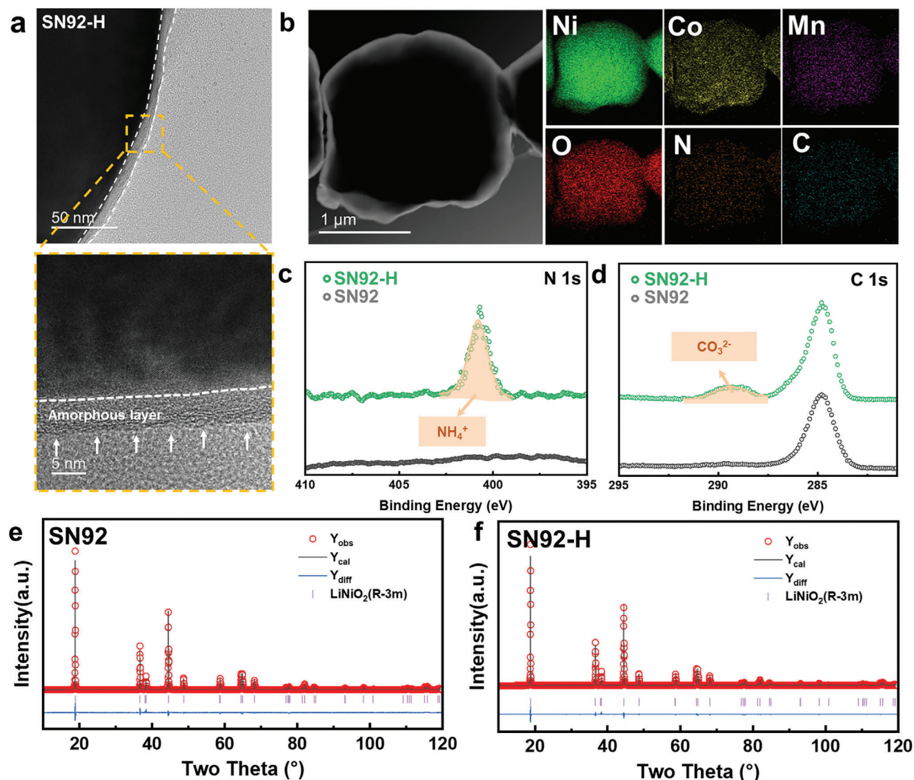
Figure 1. Construction of proton-rich shell. a) The high-resolution TEM image of SN92-H. b) The TEM-EDS mapping of SN92-H with even distribution of Ni, Mn, Co, N and O elements. c,d) The XPS spectra of N 1s (c) and C 1s (d) for SN92 and SN92-H. e,f) Powder XRD pattern and Rietveld refinement plot of SN92 (e) and SN92-H (f), respectively.
