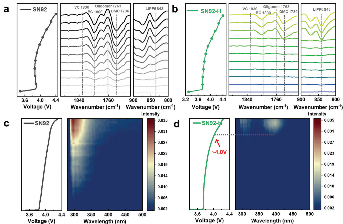
Figure 2. Characterizations of the cathode/electrolyte interface reaction in 1st cycle. a,b) Operando FT-IR difference spectra in C=O and P-F stretching region on SN92 (a) and SN92-H (b) surface during charging to 4.4 V at the initial cycle. Inserted dashed lines depict the finger peak of different compositions: VC (1830 cm -1 ), EC (1800 cm -1 ), Oligomer (1763 cm -1 ), DMC (1736 cm -1 ), LiPF 6 (843 cm -1 ). c,d) In situ UV spectra of electrolyte within SN92 (c) and SN92-H (d) half cell during charging to 4.3 V at the first cycle.
