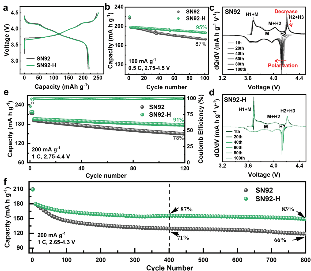
Figure 4. Electrochemical performance. a) Charging and discharging curves of SN92 and SN92-H at the first cycle. b) Cycling stability for SN92 and SN92-H half cells within the voltage range of 2.75–4.5 V at 0.5 C. c,d) Corresponding dQ/dV profile of the 1st, 20th, 40th, 60th, 80th, and 100th cycle for SN92 (c) and SN92-H (d). e) Cycling stability for SN92 and SN92-H half cells within the voltage range of 2.75–4.4 V at 1 C. f) Cycling performance of full cells with SN92 or SN92-H as cathode and graphite as anode within the voltage range of 2.65–4.3 V at 1 C.
