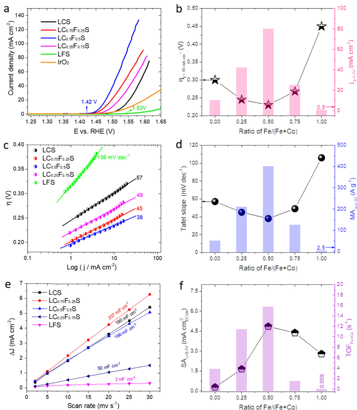
Fig. 2. Electrocatalytic activities of LC_xFe_{1-x}S ( 0 \leq x \leq 1 ) samples for OER. (a) Polarization LSV curves at 1.0 \text{ mV s}^{-1} in 1 \text{ M KOH} electrolyte, (b) comparison of overpotential at current density of 10 \text{ mA cm}^{-2} and current density at overpotential of 0.3 \text{ V} , (c) Tafel plots, (d) comparison of Tafel slope and mass activity at overpotential of 0.3 \text{ V} , (e) charging current density differences ( \Delta J = J_a - J_c ) plotted versus scan rate. The linear slope, equivalent to twice the double-layer capacitance C_{dl} , was used to represent the ECSA, (f) comparison of specific activity and TOF at overpotential of 0.3 \text{ V} .
